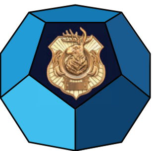
Dodecahedron
