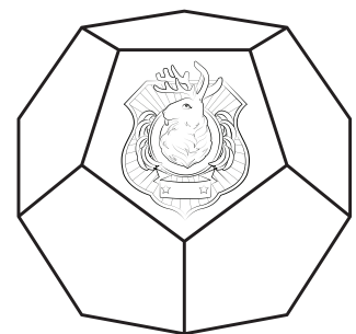
Dodecahedron
