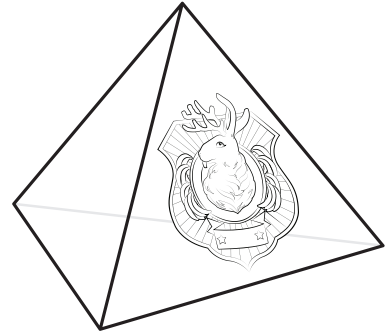
Tetrahedron
